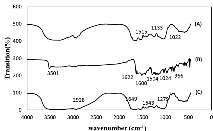
FIGURE 1 FTIR spectrums of CUR-microalga (A), CUR (B), and microalga (C)
