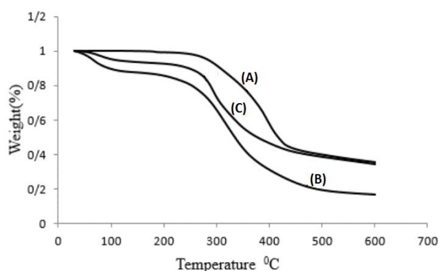
FIGURE 2 Thermal analysis of CUR (A), microalga (B), and microalga-CUR microcapsules (C)
