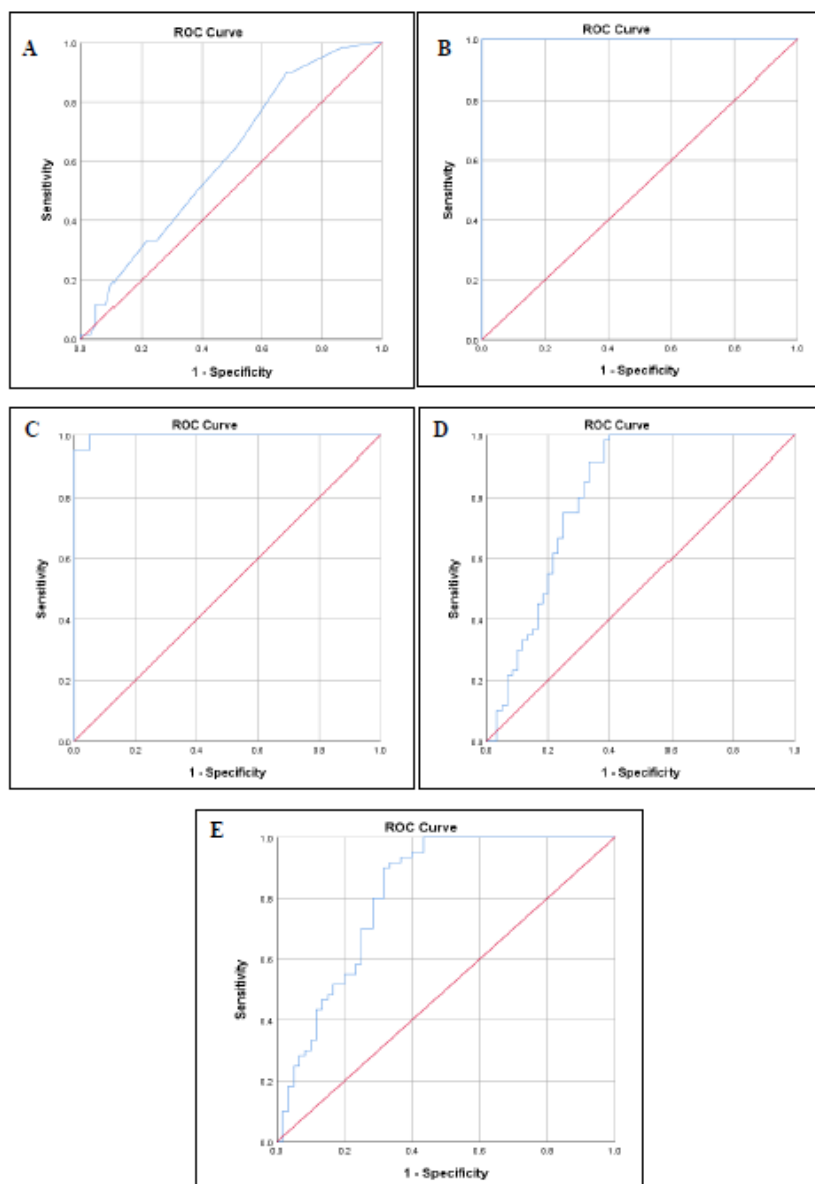
FIGURE 2 The ROC of TOC (A), TAC (B), OSI (C), CAT (D), and CAT specific activity (E) in differentiation between newly diagnosed BC and TAM-treated patients
