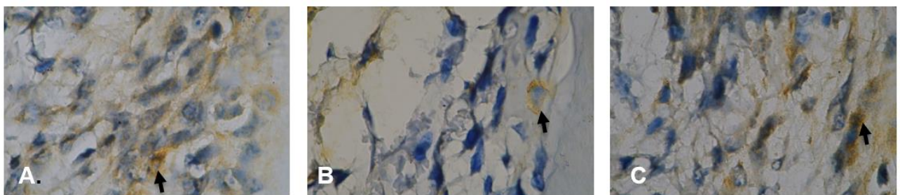
FIGURE 3 HSP10 expression in dental pulp macrophage cells in control group (A), in normal pulp tissue extirpation group (B), and in inflamed pulp tissue extirpation group (C) at 1000x magnification
